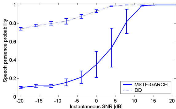
Figure 2: Conditional speech presence probability obtained by the proposed algorithm and by the decision-directed based algorithm.
