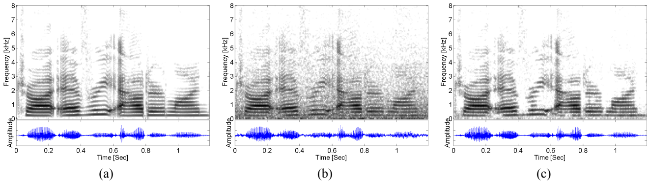
Figure 1: Speech spectrograms and waveforms. (a) Clean signal: "Try any other line."; (b) speech corrupted by factory noise with 5 dB SNR (LSD= 6.68 dB, SegSNR= 0.05 dB); (c) speech reconstructed by using 4-state model (LSD= 3.14 dB, SegSNR= 6.76 dB).
